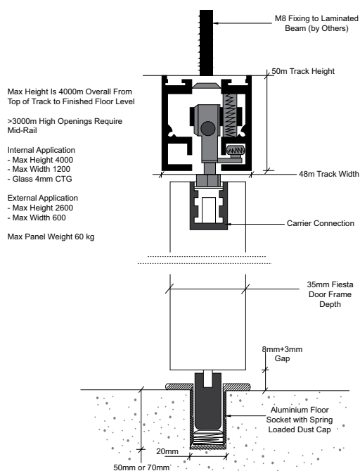
Single Stack 90° & Parallel Stack Section
